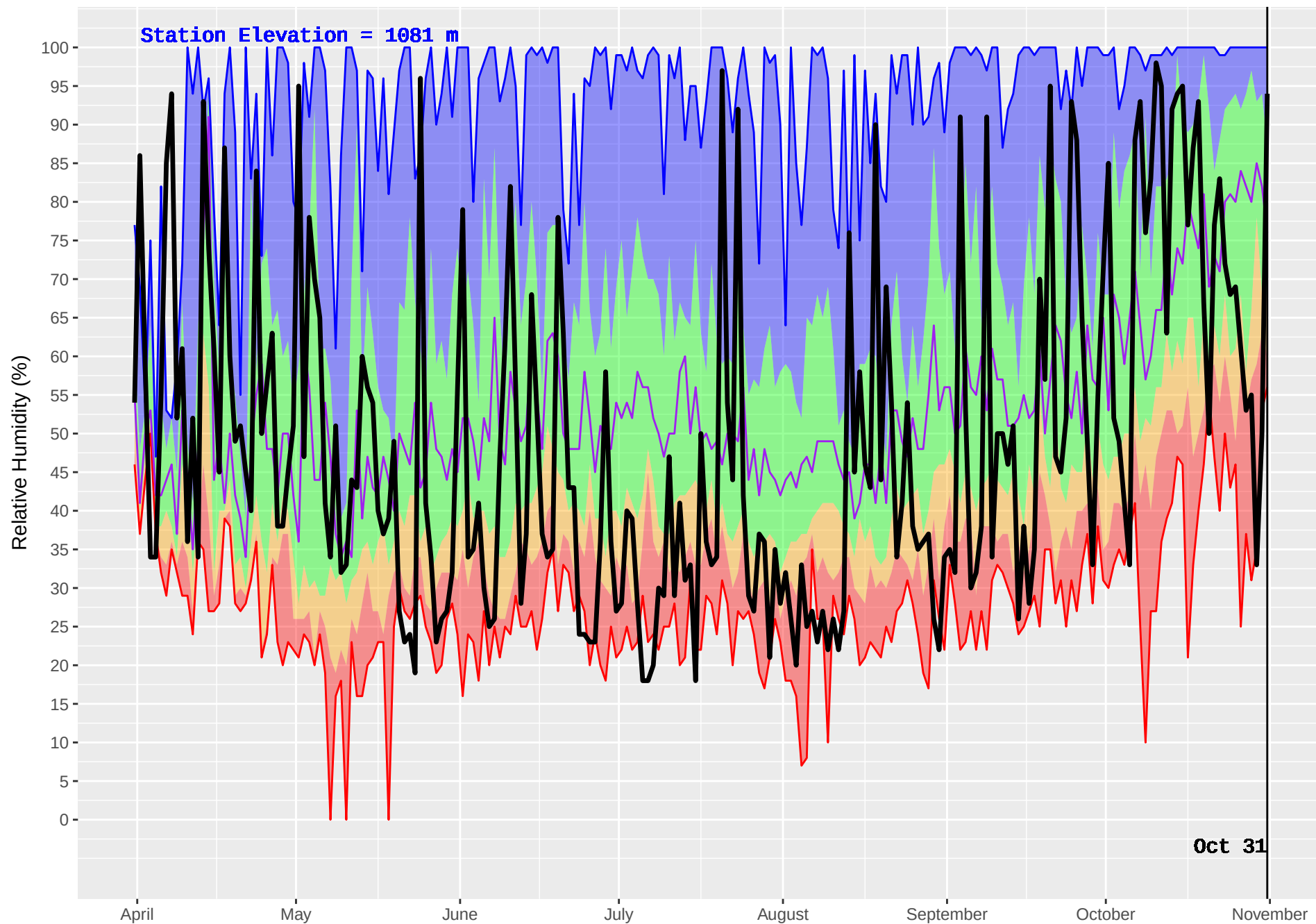
GAVIN (227) : Historical (1981–2016) and Current (2017) Noon Relative Humidity
