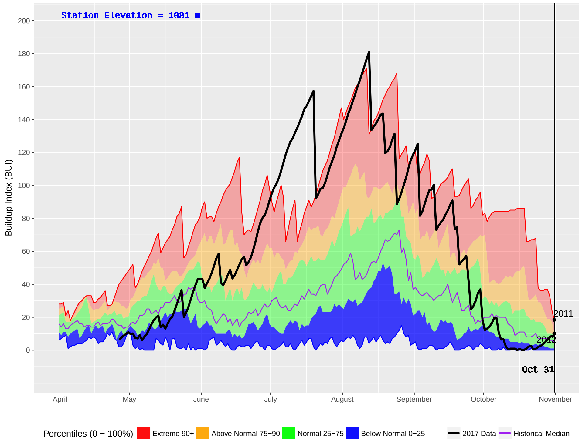
GAVIN (227) : Historical (1981–2016) and Current (2017) Noon Buildup Index (BUI)
