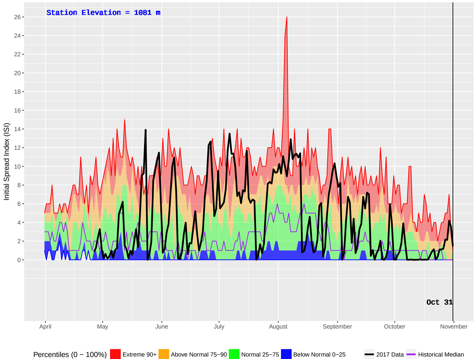
GAVIN (227) : Historical (1981–2016) and Current (2017) Noon Initial Spread Index (ISI)
