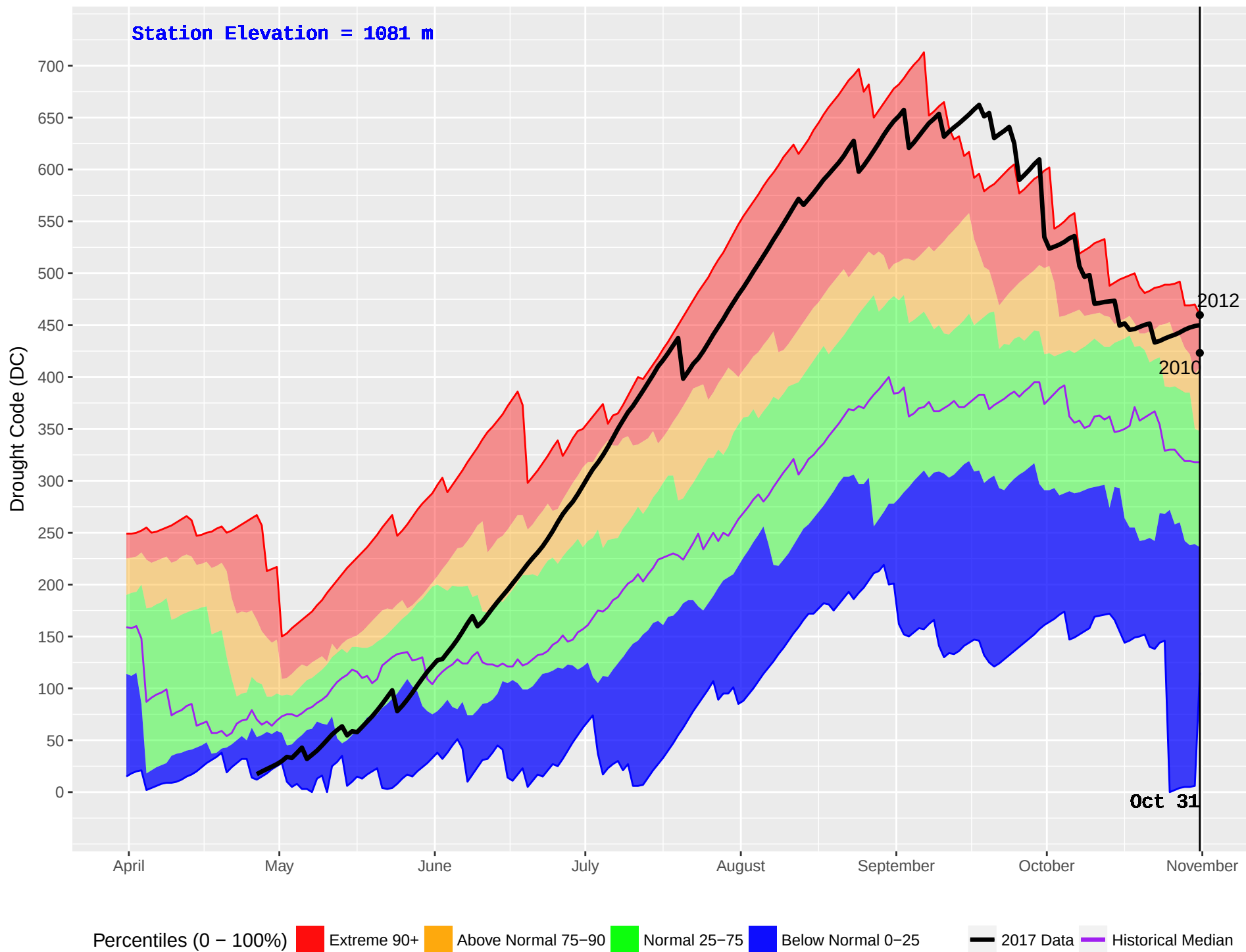
GAVIN (227) : Historical (1981–2016) and Current (2017) Noon Drought Code (DC)
