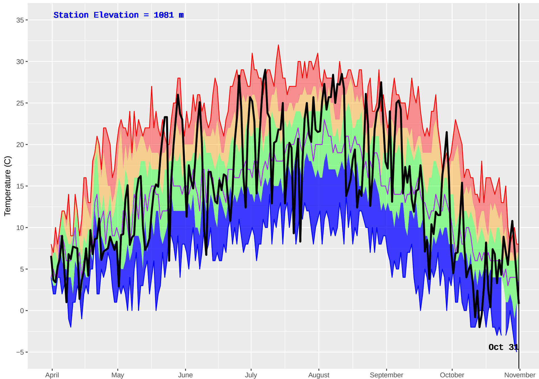
GAVIN (227) : Historical (1981–2016) and Current (2017) Noon Temperature
