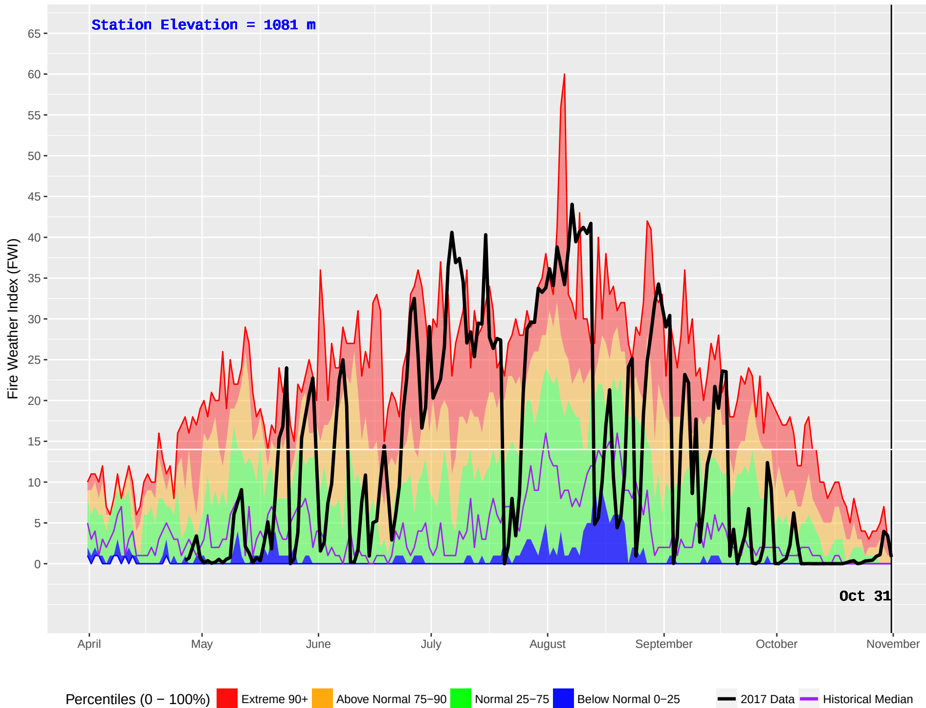
GAVIN (227) : Historical (1981–2016) and Current (2017) Noon Fire Weather Index (FWI)
