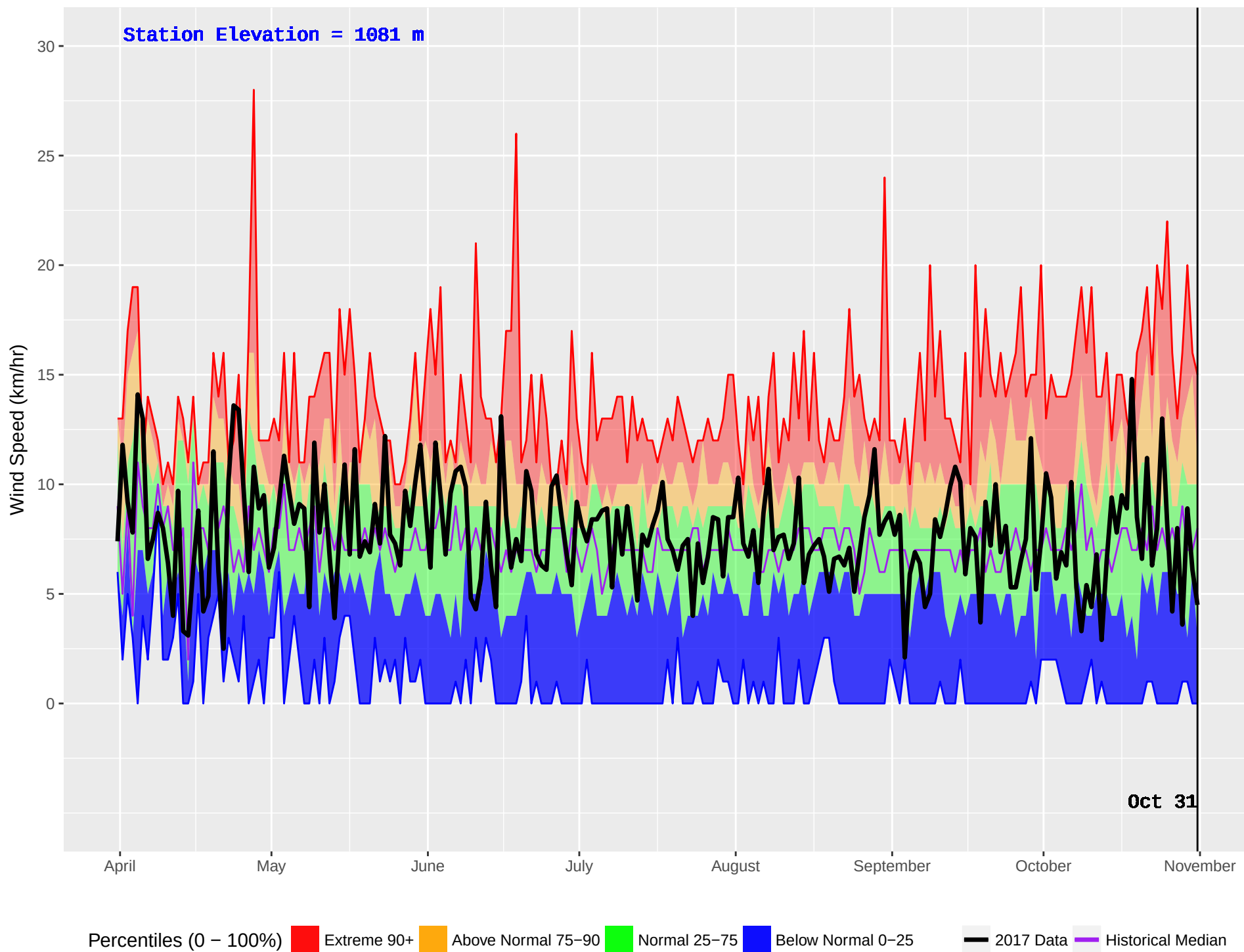
GAVIN (227) : Historical (1981–2016) and Current (2017) Noon Wind Speed
